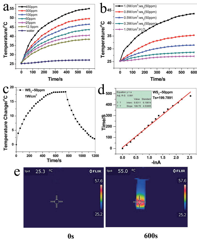
Fig. 2 (a) Temperature evaluation of pure water and the aqueous dispersion of \text{WS}_2 nanosheets at different concentrations (12.5, 25, 50, 100, 300, 450 ppm) as a functional of irradiation time (0–10 min) using an 808 nm laser at a power density of 1.0 \text{ W cm}^{-2} at room temperature. (b) Temperature evaluation of the aqueous dispersion of \text{WS}_2 nanosheets (50 ppm) as a functional of irradiation time (0–10 min) using an 808 nm laser at different power densities ( 0.3, 0.5, 0.8, 1.0 \text{ W cm}^{-2} ), and pure water was used as the negative control. (c) Photothermal response of the aqueous dispersion of \text{WS}_2 nanosheets (50 ppm) under the NIR laser (808 nm, 1.0 \text{ W cm}^{-2} ) irradiation for 13 min, and then the laser was shut off. (d) Linear time data versus -\ln \theta obtained from the cooling period of (d). (e) IR images of the \text{WS}_2 nanosheets solution before and after the 808 nm laser irradiation at a power density of 1 \text{ W cm}^{-2} for 10 min.
