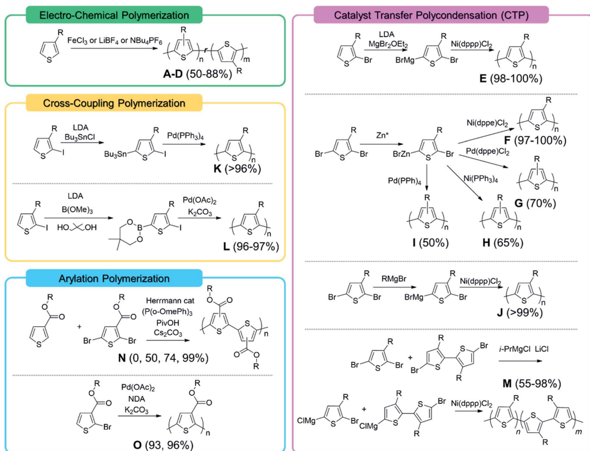
Fig. 2 Synthesis of P3ATs with different RRs via various methods: electro-chemical polymerization, 54–56 cross-coupling polymerization, 75,76 arylation polymerization, 75,76 and catalyst transfer polycondensation. 25,60–63,74
