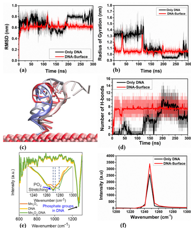
Fig. 5 The presence of a surface significantly affects the ssDNA structure. Variation of (a) RMSD, and (b) radius of gyration during the course of simulation. (c) A snapshot of the system showing unfolding and folding of ssDNA between 30 and 38 ns. Water molecules have been removed for clarity. The surface is illustrated with VdW spheres with colour code: pink: Mn, red: O. ssDNA is presented using a “new Cartoon” representation scheme of VMD with colour code: red: folded ssDNA at 30 ns; white: intermediate unfolded ssDNA; and blue: folded ssDNA at 38 ns. (d) Temporal variation of intramolecular H-bonds in the presence and absence of surface. (e) Experimental FTIR spectrum of DNA and (f) computed power spectrum of the phosphate groups of ssDNA. (e) Inset illustrates the experimentally observed changes of FTIR spectrum of phosphate group of DNA in presence of \text{Mn}_3\text{O}_4 .
