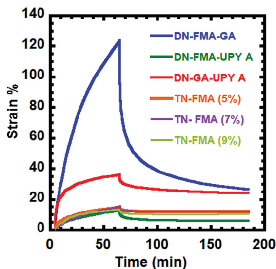
Fig. 5 Creep and creep recovery curves of all materials by applying 5 kPa stress for 1 h and 2 h for recovery.
