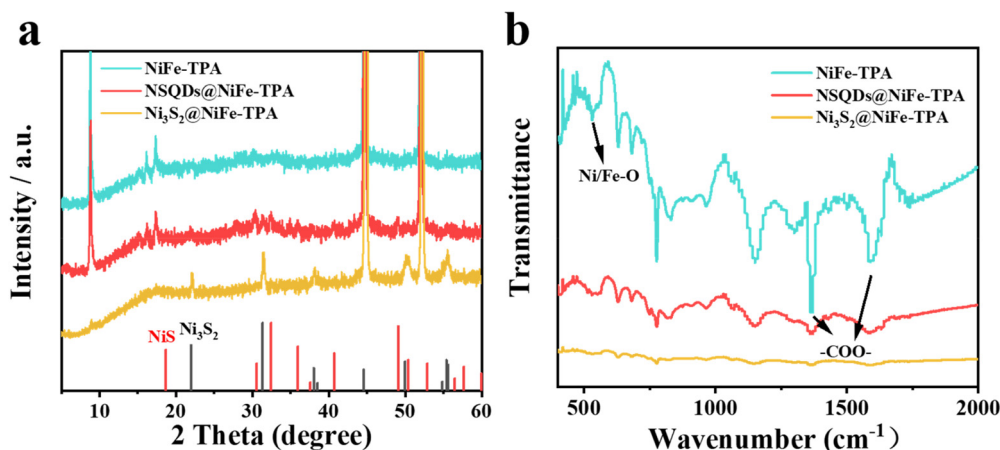
Fig. 2 (a) XRD patterns and (b) FT-IR spectra of NiFe-TPA, NSQDs@NiFe-TPA and \text{Ni}_3\text{S}_2 @NiFe-TPA.
