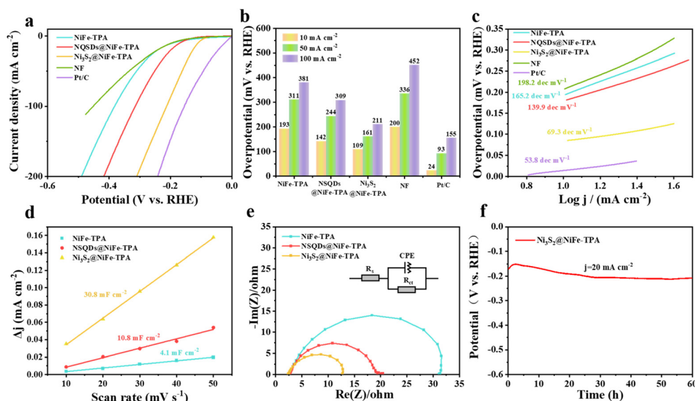
Fig. 5 (a) LSV curves, (b) comparison of the overpotentials, (c) Tafel plots derived from LSV curves, (d) double-layer capacitance ( C_{dl} ) plots of NiFe-TPA, NSQDs@NiFe-TPA, \text{Ni}_3\text{S}_2 @NiFe-TPA, NF and Pt/C, (e) Nyquist plots of NiFe-TPA, NSQDs@NiFe-TPA and \text{Ni}_3\text{S}_2 @NiFe-TPA, (f) chronopotentiometry (CP) curve of \text{Ni}_3\text{S}_2 @NiFe-TPA at a current density of 20 \text{ mA cm}^{-2} .
