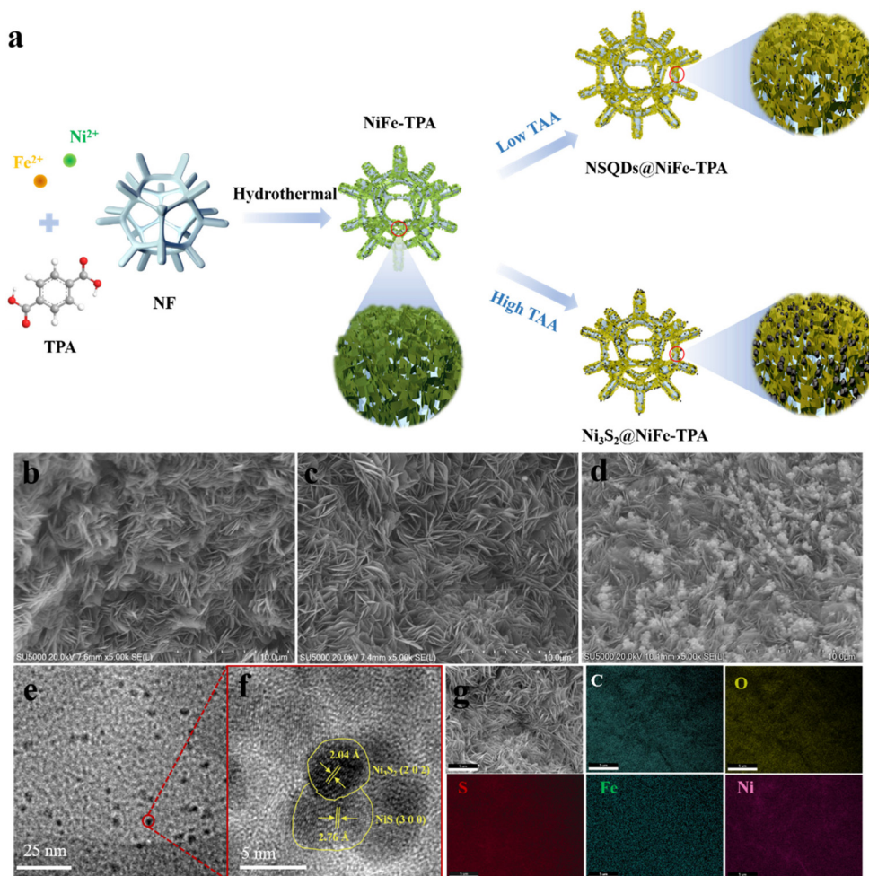
Fig. 1 (a) Schematic diagram of the synthesis process of NiFe-TPA, NSQDs@NiFe-TPA and \text{Ni}_3\text{S}_2 @NiFe-TPA. SEM images of (b) NiFe-TPA, (c) NSQDs@NiFe-TPA and (d) \text{Ni}_3\text{S}_2 @NiFe-TPA, (e and f) HRTEM images of NSQDs@NiFe-TPA, and (g) EDX mapping of NSQDs@NiFe-TPA.
