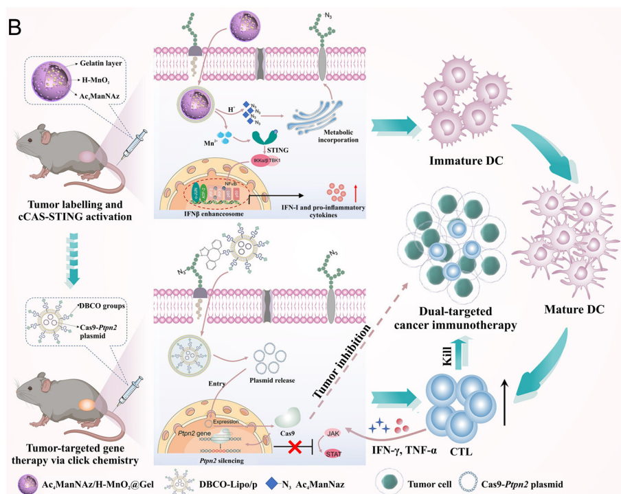
Fig. 5 Editing of the Ptpn2 gene in tumor cells for cancer immunotherapies. (A) The construction of HPR@CCP nanoparticles and their versatile application in cancer combined therapy. 168 (B) Process of the selective labeling of tumor tissues via metabolic engineering by Ac 4 ManNAz/H-MnO 2 @Gel, and the illustration of the targeted CRISPR/Cas9 system delivery and tumor-specific gene editing of Ptpn2 by DBCO-Lipo/p via biorthogonal click chemistry. 169
