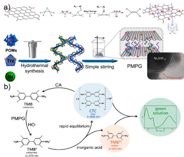
Fig. 4 Applications of the \text{Ni}_4\text{SiW}_{12} /PDDA-rGO in the detection of CA. (a) Schematic illustration of synthesizing \text{Ni}_4\text{SiW}_{12} /PDDA-rGO. (b) Schematic illustration of detecting CA using \text{Ni}_4\text{SiW}_{12} /PDDA-rGO. 29 Copyright 2020, Elsevier.
