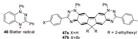
Fig. 13 Chemical structures of a Blatter radical and derivatives.
