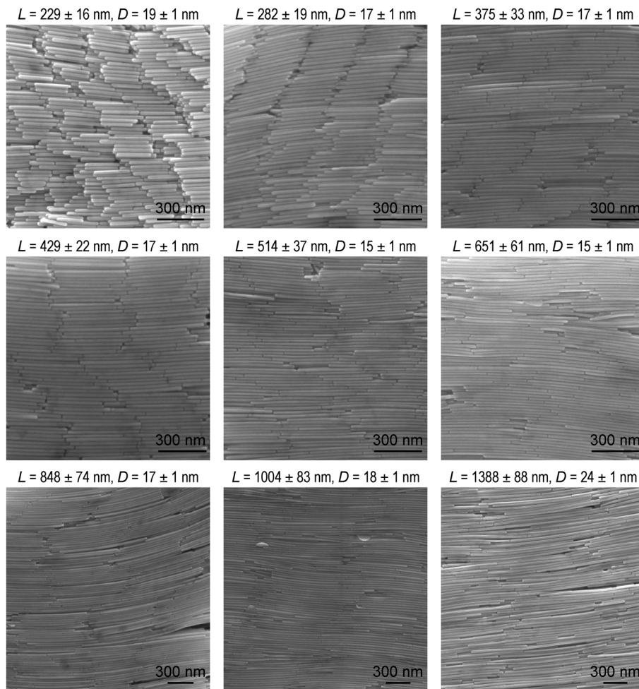
Fig. 1 SEM images of the purified Au nanorod samples with different dimensions. The average length and diameter of each sample are indicated above the corresponding SEM image.
