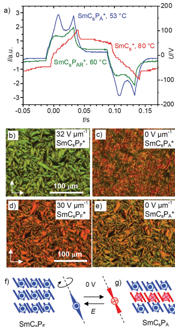
Fig. 8 (a) Switching current response curves of compound ( S )-2/12 at 80 °C (SmC s *), 60 °C (SmC s P AR *) and 53 °C (SmC s P A *), respectively, under a triangular wave field (380 V pp , 50 Hz, 5 kΩ); (b) and (c) planar textures as observed between crossed polarizers at 65 °C, and (d) and (e) at 53 °C in a 10 μm non-coated ITO cell; (f) and (g) models showing the helix-free SmC s P F and SmC s P A structures and the switching between them by rotation around the molecular long axis.
