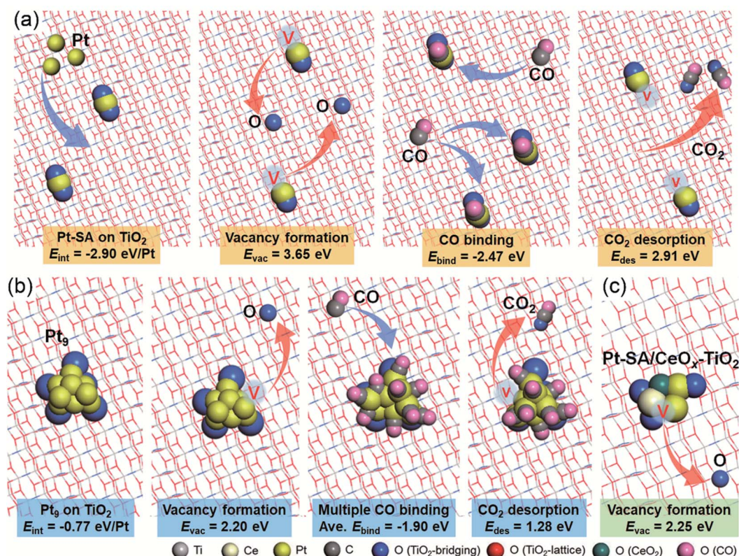
Fig. 3 Long-term CO DFT-estimated interface chemistry of Pt catalysts. (a) Pt-SA on TiO 2 , (b) Pt 9 on TiO 2 , and (c) Pt-SA on CeO x -TiO 2 . The E_{\text{int}} denotes the normalized Pt-TiO 2 interaction energy. E_{\text{vac}} and E_{\text{des}} correspond to the energy of oxygen vacancy formation and the energy of CO 2 desorption (production), respectively. E_{\text{bind}} is the energy of CO binding on Pt. The averaged E_{\text{bind}} of total 9 CO molecules is presented in (b).
