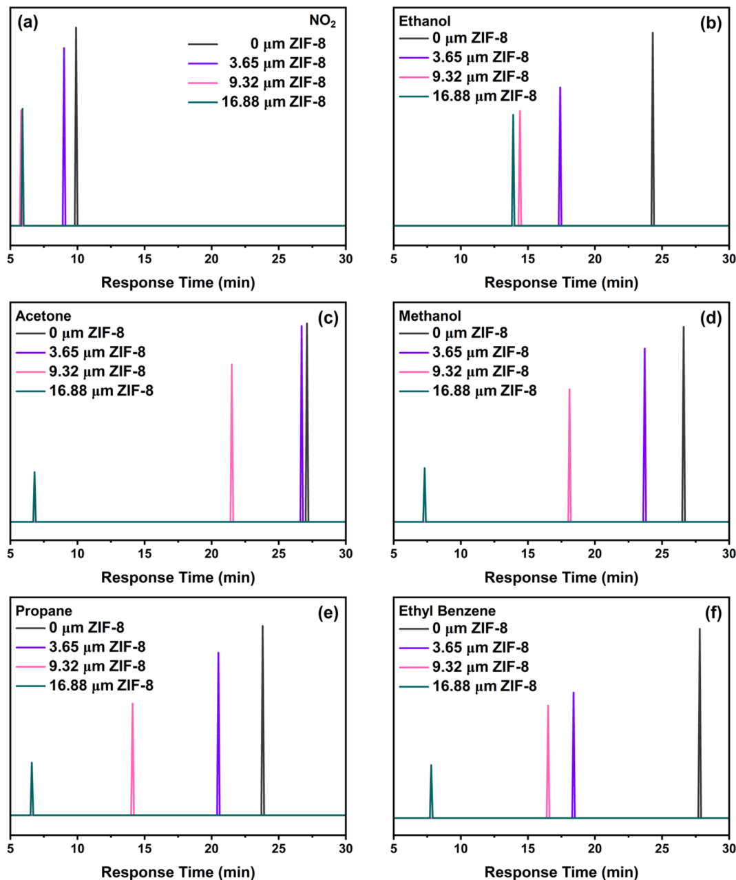
Fig. 6 Response time profiles of the developed sensors with different ZIF-8 thickness: 0 μm (grey), 3.65 μm (purple), 9.32 μm (pink) and 16.88 μm (green) against various target gases (a) NO 2 , (b) ethanol (c) acetone (d) methanol (e) propane (f) ethyl benzene.
