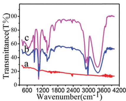
Fig. 3 FTIR spectra of (a) FePt, (b) FePt-CH=CH 2 and (c) NIPAM grafted FePt nanoclusters.
