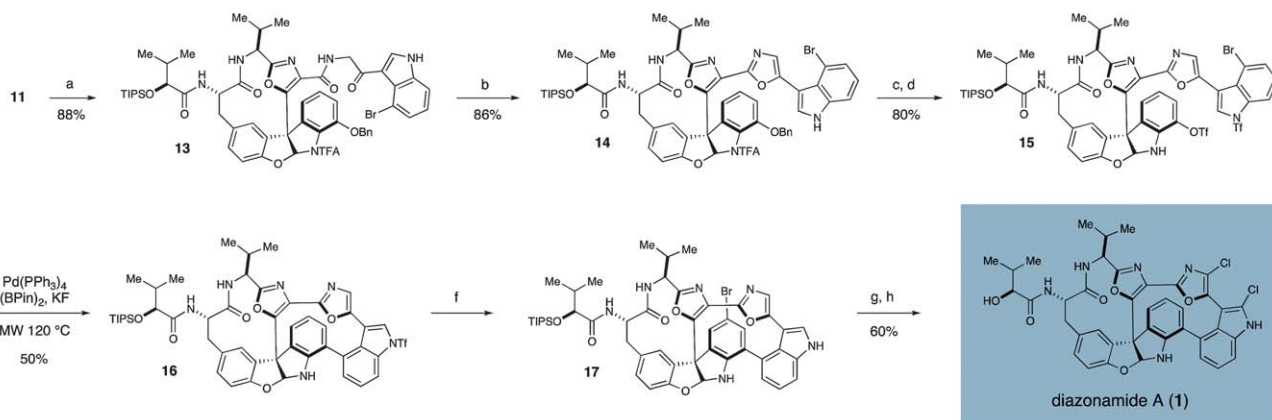
Scheme 2 Construction of the second macrocyclic ring, dichloro installation and completion of the total synthesis of diazonamide A ( 1 ). Reagents and conditions: (a) AgTFA, NaHCO 3 , 2-amino-1-(4-bromo-1 H -indol-3-yl)ethanone·TFA, DMF, 40 °C (b) PPh 3 , C 2 Cl 2 , NEt 3 , CH 2 Cl 2 , 0 °C (c) BBr 3 , CH 2 Cl 2 , -78 °C (d) PhNTf 2 , NEt 3 , CH 2 Cl 2 , rt (e) (Bpin) 2 , KF, 70 mol% Pd(PPh 3 ) 4 , dioxane:H 2 O (20 : 1), MW 120 °C (f) NBS, THF; then LiOH, THF, MeOH, H 2 O (g) NCS, THF, 40 °C; then H 2 , Pd(OH) 2 , THF, 40 °C (h) TASF, DMF, rt.
