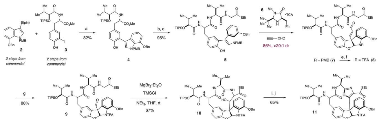
Scheme 1 Organocatalytic synthesis of the furanoindoline core and Lewis acid mediated synthesis of left-hand macrocycle of diazonamide A. Reagents and conditions: (a) 5 mol% Pd(dppf)Cl 2 , K 3 PO 4 , dioxane, 40 °C (b) LiOH, THF, MeOH, H 2 O, rt (c) EDC, HOBt, ( S )- S -ethyl 2-(2-amino-3-methylbutanamido)ethanethioate·TFA, NaHCO 3 , DMF, rt (d) Table 1, entry 5 (e) DDQ, CH 2 Cl 2 , pH 7 buffer, 0 °C (f) TFAA, DMAP, CH 2 Cl 2 , 0 °C (g) O 3 , CH 2 Cl 2 , MeOH, −78 °C (h) MgBr 2 ·Et 2 O, TMSCl, NEt 3 , THF, rt (i) Dess–Martin, CH 2 Cl 2 , rt (j) DAST, C 6 H 6 , rt.
