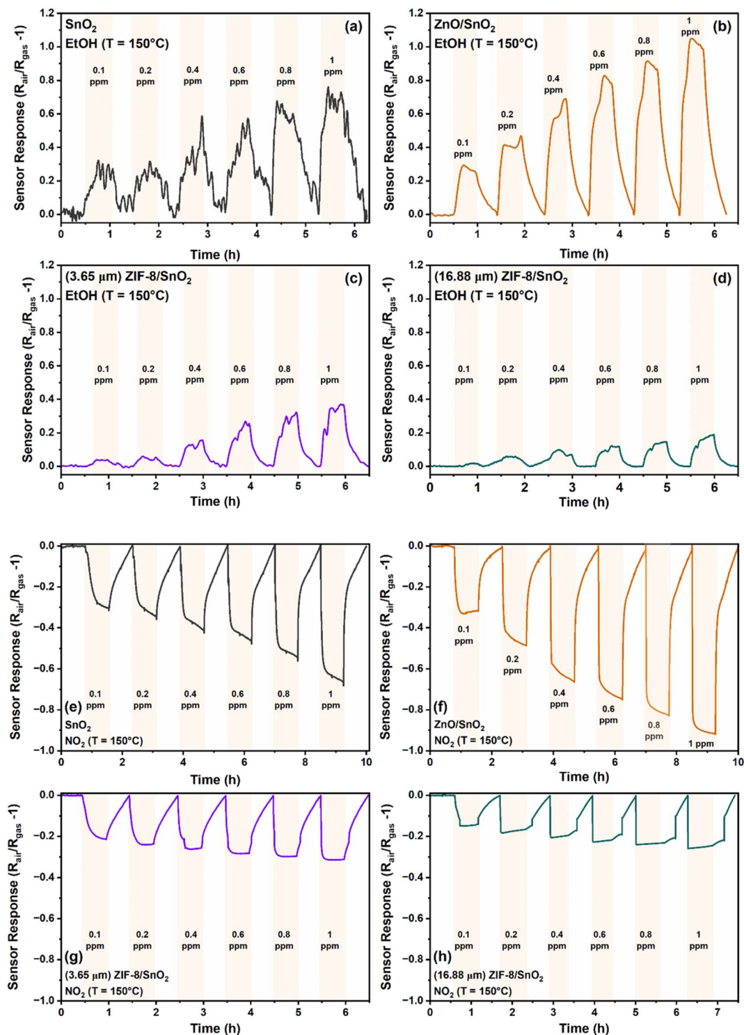
Fig. 3 Dynamic sensing of a pure \text{SnO}_2 layer (black), \text{ZnO}/\text{SnO}_2 dual layer (brown), 3.65 \mu\text{m} \text{ZIF-8}/\text{SnO}_2 (purple) and 16.88 \mu\text{m} thick \text{ZIF-8}/\text{SnO}_2 (green) dual layer under exposure to increasing concentrations of ethanol, a reducing gas (a–d) and \text{NO}_2 , an oxidizing gas (e–h), from 0.1–1 ppm at an operating temperature of 150^\circ\text{C} .
