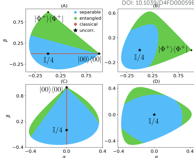
Figure 2. Left: schematic illustration of the sets of uncorrelated (black), classical (red), separable (blue) and entangled (green) states and the corresponding geometric correlation measures. Right: two-dimensional intersections of the high-dimensional set of two-qubit states. The point (\alpha, \beta) = (0, 0) represents the maximally mixed state. While in (A), (B), (C) the underlying intersecting plane contains the states |00\rangle and/or |\Phi^+\rangle = (|00\rangle + |11\rangle)/\sqrt{2} , the intersecting plane for (D) is chosen at random.
