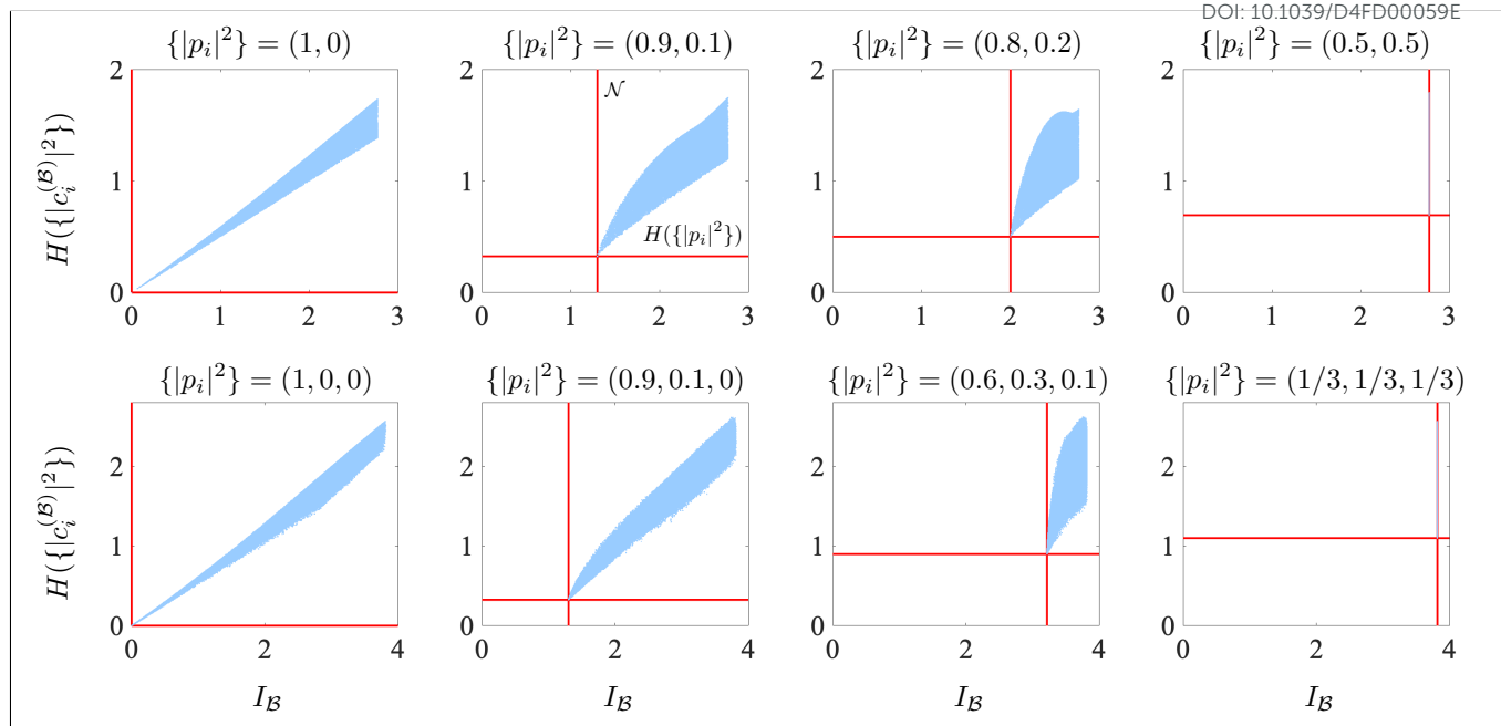
Figure 6. Relation between total orbital correlation I_B(|\Psi_{2e}\rangle\langle\Psi_{2e}|) and Shannon entropy H(\{|c_i^{(B)}|^2\}) of the CI expansion coefficients of two-electron quantum state (54) in 2K modes for numerous randomly sampled orbital reference bases \mathcal{B} . The horizontal and vertical red lines indicate the minima of the two quantities, given by H(\{|p_i|^2\}) and \mathcal{N} (nonfreeness), respectively. In the first row we set K = 2 , and in the second row K = 3 . Different plots in the same row correspond to different choices of the parameters \{|p_i|^2\}_{i=1}^K in (54) that uniquely determine the multireference structure of the state.
