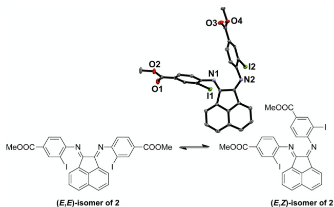
Figure 1. ( E,E )- and ( E,Z )-isomeric forms of 2 .
