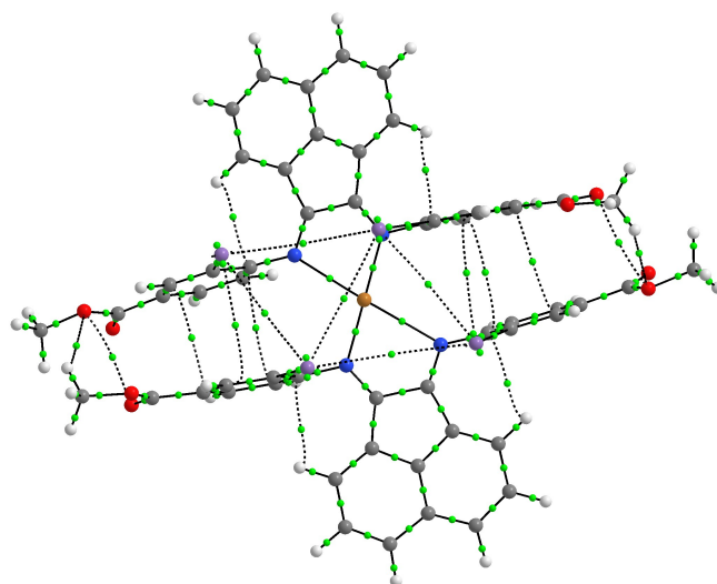
Figure 6. AIM plot for 4 in toluene, with the light-green points being BCPs.
