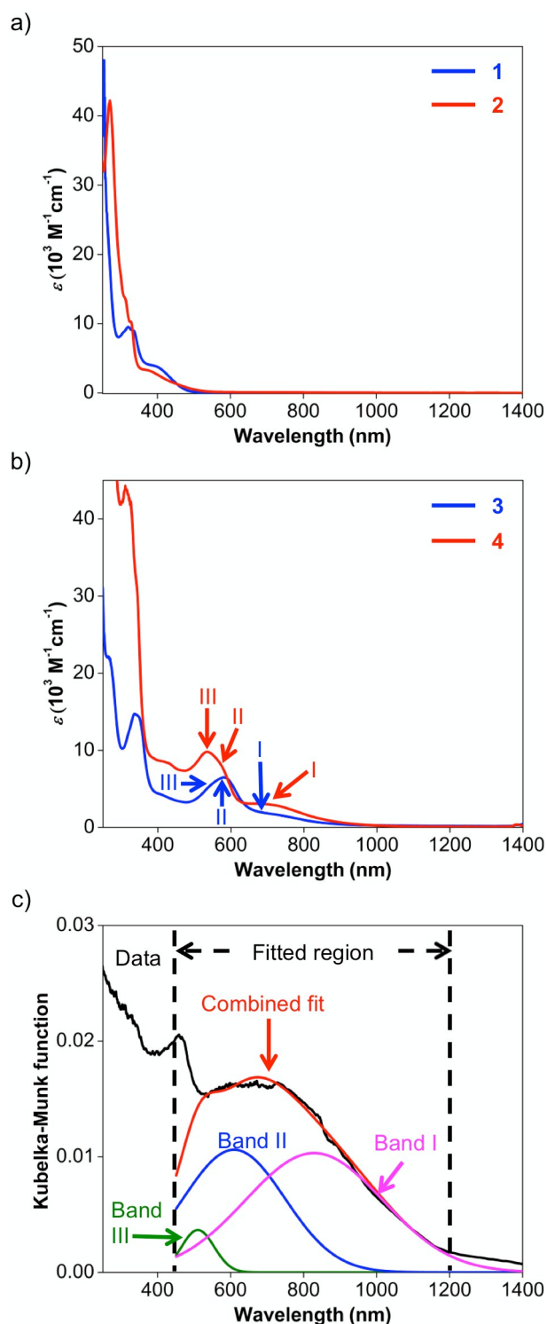
Figure 4. (a) UV-visible spectra of 1 (blue) and 2 (red) in methanol and DCM respectively. (b) UV-visible spectra of 3 (blue) and 4 (red) in methanol and DCM respectively. Roman numerals and arrows indicate the wavelength for the various fitted absorption bands of 3 (blue) and 4 (red). (c) Diffuse reflectance spectrum of 4 with fits for bands I (pink), II (blue), and III (green). The black line corresponds to the experimental data, while the red line is the superposition of the fitted bands.
