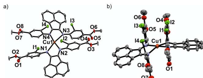
Figure 2. Oak Ridge Thermal Ellipsoid Plots (ORTEPs) from single crystal X-ray diffraction experiments of 4 . Top (a) and side views (b) of crystals grown from THF/toluene. The \text{PF}_6^- counteranion and the calculated hydrogen atoms are omitted for clarity.
