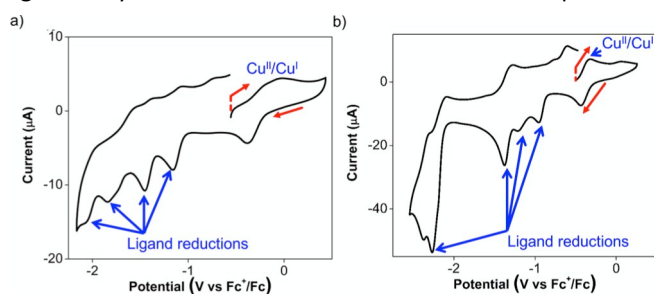
Figure 3. Cyclic voltammograms of (a) 1.0 mM of 3 and (b) 1.0 mM of 4 in DMF/DMSO 1:1 (v:v), with 0.10 M n -Bu 4 NBARF 4 as the electrolyte, each at a scan rate of 100 mV s -1 with its scan direction and initial potential indicated by the red arrows and red vertical dashed line respectively. The data are reported relative to Fc + /Fc.
