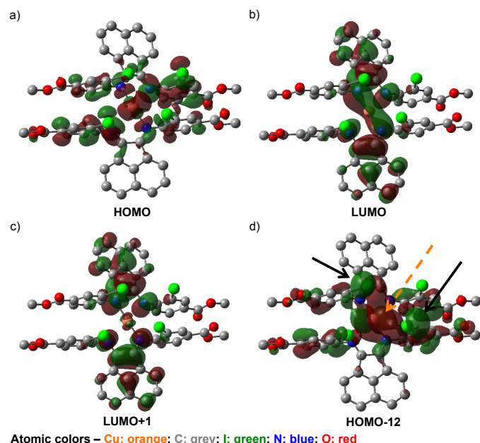
Figure 5. (a) HOMO, (b) LUMO, and (c) LUMO+1 of geometry-optimized 4 in toluene, set at isovalues of 0.02, and (d) HOMO-12 set at an isovalue of 0.01. The orange arrows in (d) indicate the d orbital lobe contributions from Cu(I), while the black arrows point to the p-orbital contributions from two of the iodides in 2 .
