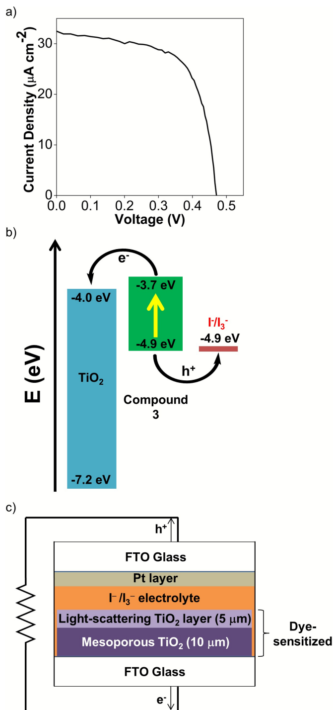
Figure 7. (a) J-V plot for DSSCs after 3 has been adsorbed for dye-sensitization. (b) Band alignment for DSSC incorporated with 3 , showing the relative energy levels (in eV against vacuum) for 3 , TiO 2 , and the I - /I 3 - electrolyte. (c) General device structure for the DSSCs prepared in this study.
