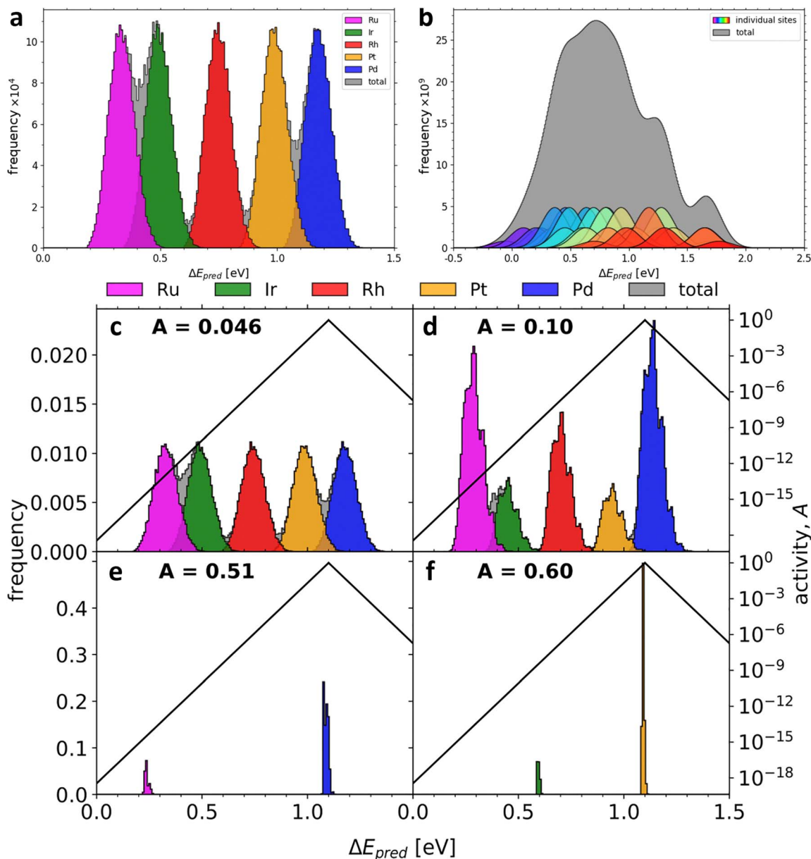
Fig. 8 (a) and (b) Predicted adsorption energies for \text{OH}^* and \text{O}^* . (c), (d), (e), and (f) Distributions of the adsorption energies for IrPdPtRhRu, Ir 10.2 Pd 32 Pt 9.3 Rh 19.6 Ru 28.9 , Pd 81.7 Ru 18.3 and Ir 17.5 Pt 82.5 , respectively. Reproduced with permission. 56 Copyright 2019, Cell Press.
