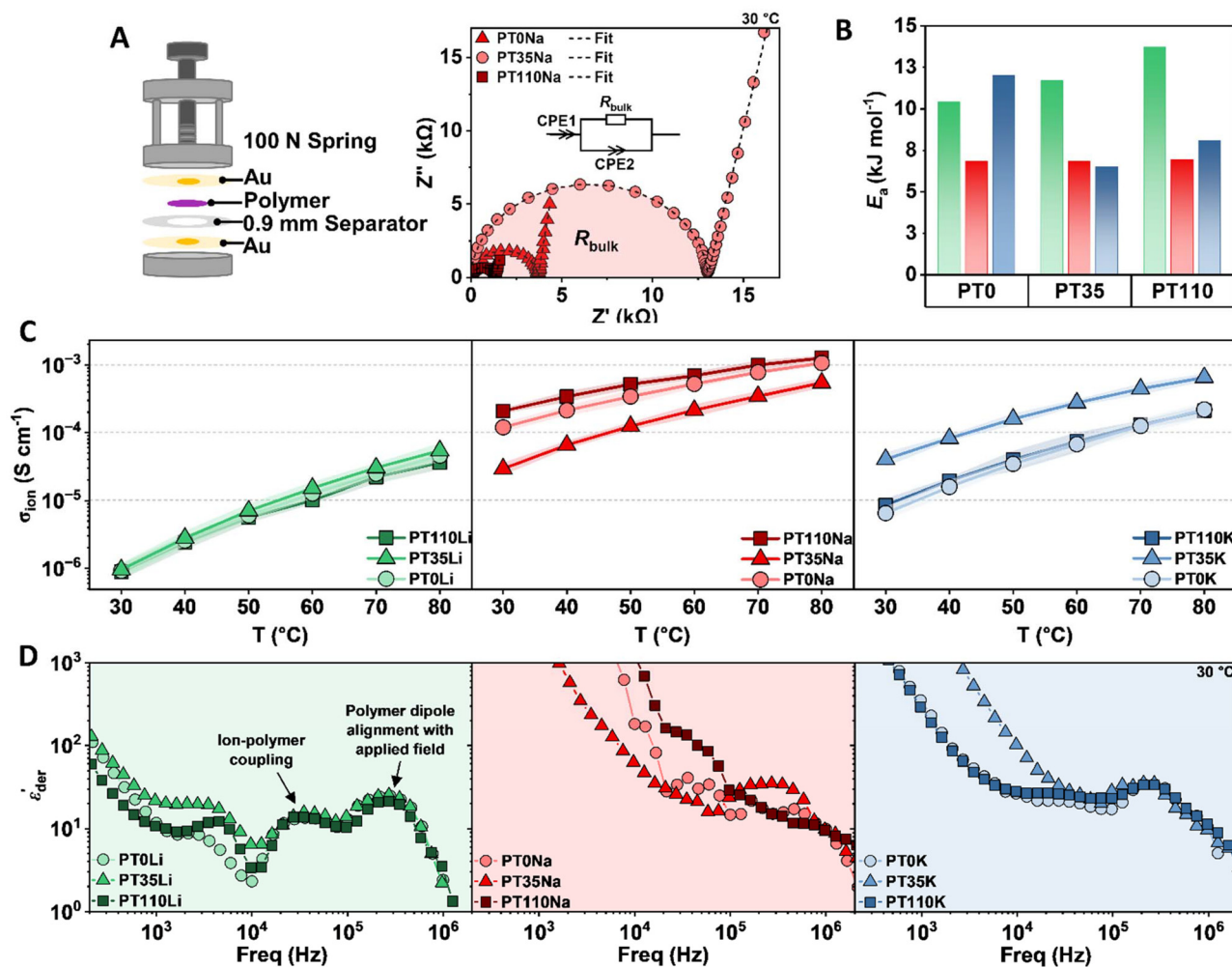
Fig. 3 Ionic transport. (A) Cell set-up for electrochemical impedance spectroscopy (EIS) with gold blocking electrodes, and representative Nyquist plots for Na + series showing the equivalent circuit used to determine bulk resistance (data fit). (B) Activation energies calculated from VTF fits of the temperature-dependent ionic conductivity data shown in (C). (D) Dielectric relaxation spectra (DRS) probing frequency-dependent relaxations and ionic processes.
