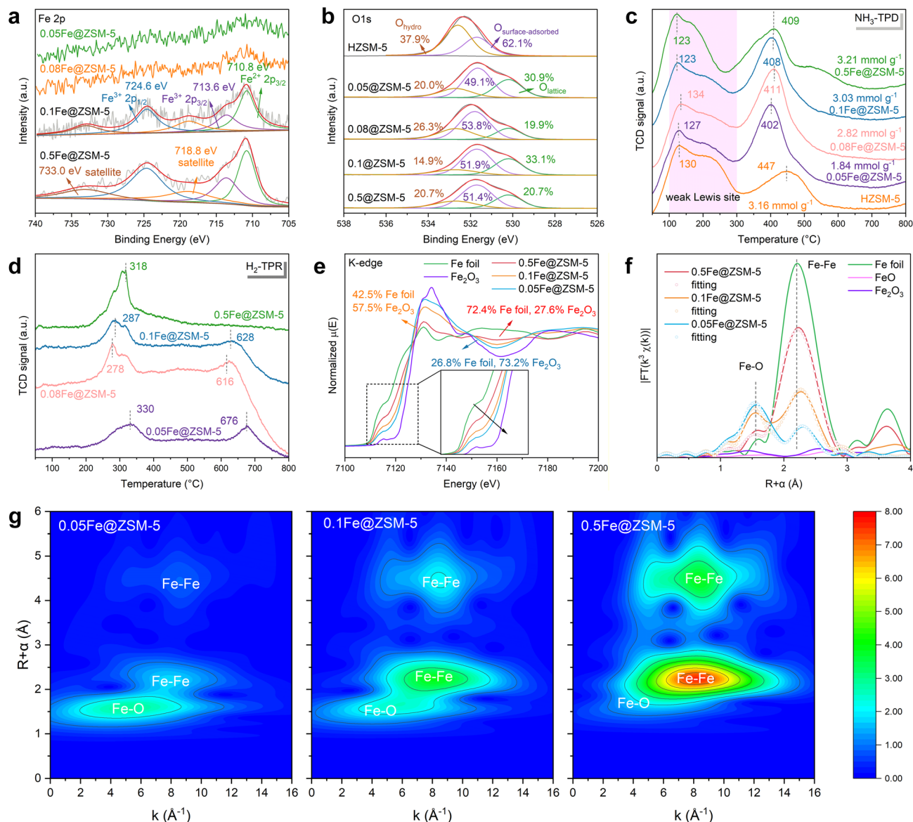
Fig. 2 Electronic state and coordination structure characterization on Fe@ZSM-5. (a) Fe 2p spectra; (b) O 1s XPS spectra; (c) NH 3 -TPD spectra; (d) H 2 -TPR spectra; (e) K-edge XANES spectra; (f) K-edge EXAFS spectra; (g) Fe wavelet transforms. All FT and WT signals in this study are non-phase corrected.
