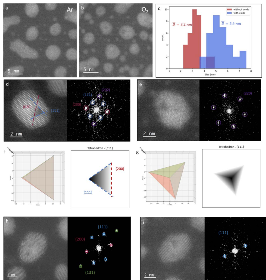
Fig. 6 HAADF-STEM images showing the voids formed in the NPs when the NPs are exposed to oxygen at 200 °C. (a) NPs under Ar before \text{O}_2 exposure and (b) under \text{O}_2 . (c) Size distribution of NPs with and without voids. (d) and (e) High-resolution HAADF-STEM images of NPs presenting a triangular-shaped void along the [110] and [111] zone axes, respectively. (f) and (g) Tetrahedral 3D models bounded by {111} facets observed along the [110] and [111] zone axes, respectively. The contrast-inverted STEM image of the tetrahedral 3D model calculated by kinematic STEM simulation; the two zone axes are shown alongside. The STEM intensity is inversely proportional to the local thickness upon contrast reversal. (h) and (i) High-resolution HAADF-STEM images of NPs containing multiple triangular-shaped voids. For stability and in order to keep the spatial resolution, high-resolution images were acquired under vacuum at room temperature.
