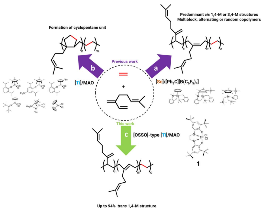
Scheme 1 Myrcene–ethylene copolymerizations: (a) promoted by Sc-based complexes (Guo and Hou); 28 (b) promoted by Ti and Zr half-metalloccenes and metallocenes; 31 (c) promoted by an [OSSO]-type bis(phenolate) Ti complex ( 1 ) (this study).
