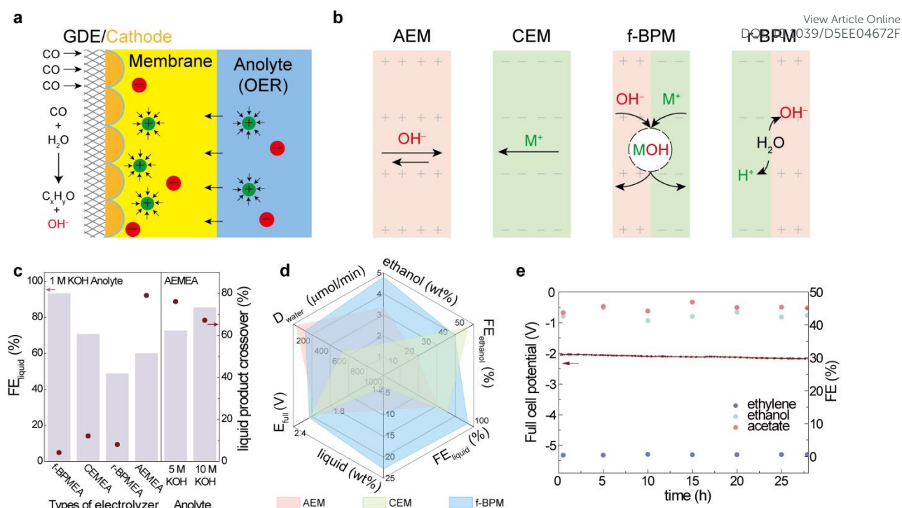
Figure 1. MEA-CO electrolyzer configuration and membrane-dependent CORR performance. a. Schematic illustrations of the interface structure in the MEA. b. Transport of ionic species ( \text{M}^+ = \text{Li}^+, \text{Na}^+, \text{K}^+, \text{Cs}^+ etc.) in different membrane configurations: anion exchange membrane (AEM), cation exchange membrane (CEM), forward-bias bipolar membrane (f-BPM) and reverse-bias bipolar membrane (r-BPM). c. Faradaic efficiency and liquid-product crossover of CORR liquid products in MEA with different membrane or anolyte. (d) Key performance metrics (water migration rate, D_{\text{water}} ; FEs and concentration of ethanol and total liquid product; full cell voltages, E_{\text{full}} ) for AEM, CEM, and f-BPM cells using 1 M KOH anolyte; (e) Cell voltage and Faradaic efficiencies for CO reduction in the optimized f-BPMEA system during a 28-hour operation.
