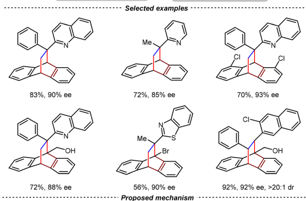
Scheme 53 Asymmetric [4+2] dearomative photocycloadditions of anthracene with alkenylazaarenes.
