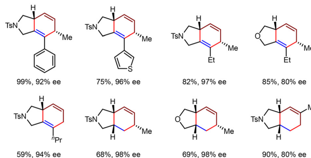
Scheme 31 \text{Co}(\text{I}) -catalyzed intramolecular [4+2] cycloaddition reactions of unactivated diene-ynes and trienes.
