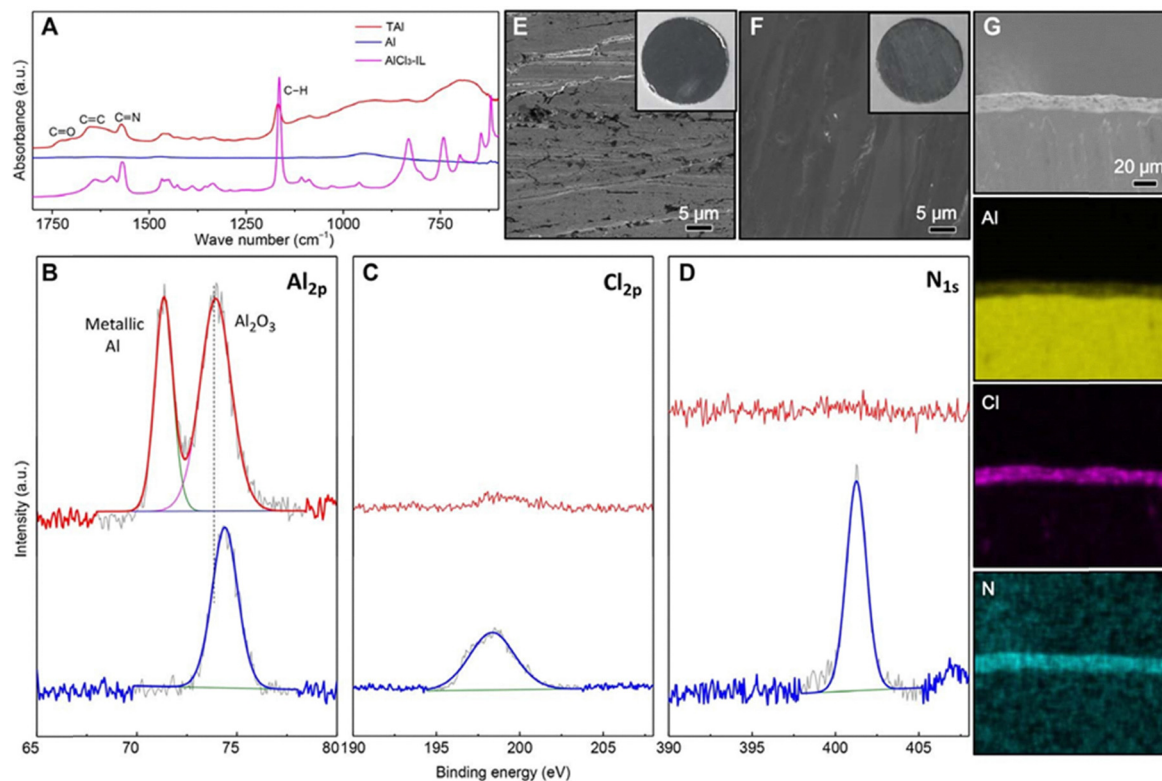
Fig. 9 Surface analysis of metal Al anode before and after treatment with \text{AlCl}_3 -IL electrolyte. (A) ATR-FTIR spectra of Al and TAl surface. XPS spectra of (B) Al 2p (C) Cl 2p (D) N 1s on Al anode (red line) and TAl anode (blue line). SEM pictures of (E) Al anode (F) TAl anode. The insets of (E) and (F) are digital image of Al and TAl (G) Cross-sectional SEM picture of TAl anode and corresponding EDX mapping of Al, Cl, and N. Al: Intact Al anode, TAl: Al anode surface treated with ionic liquid based electrolyte. a.u., arbitrary units.
