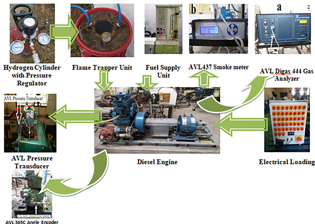
Fig. 2 Photographic view of the engine setup.
