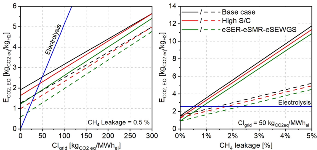
Fig. 10 E_{\text{CO}_2,\text{eq}} for the base case, high steam to carbon, and eSER–eSMR–eSEWGS plants as a function of C_{l,\text{grid}} (left) and \text{CH}_4 leakage (right). Solid lines refer to GWP20 and dashed lines to GWP100.
