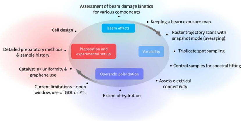
Fig. 6 Summary diagram of important considerations and recommendations for aspects affecting the successful acquisition of operando AP-XPS data on composite PEM electrolysis and fuel cells.
