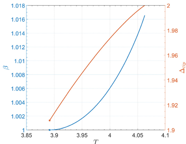
Fig. 8 Normalized crack length \beta (blue line) and \Delta_{\text{tip}} (red line) versus normalized time T for \alpha = 1.2 < \alpha^* = 1.7071 . Simulations used \beta_0 = 1 , \eta_{\text{max}} = 1 , \phi_{\text{max}} = 2 .
