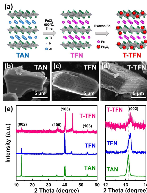
Fig. 1 (a) The schematic diagram of the synthesis process for MAX phase Ti 2 AlN (TAN), the sequential effect after Al substitution by Fe (TFN), and excess Fe toppling on TFN surface (T-TFN); (b) the modifications on the surface observed by SEM images on the TAN, (c) TFN, and (d) T-TFN; (e) XRD patterns of the TAN, TFN and T-TFN, respectively.
