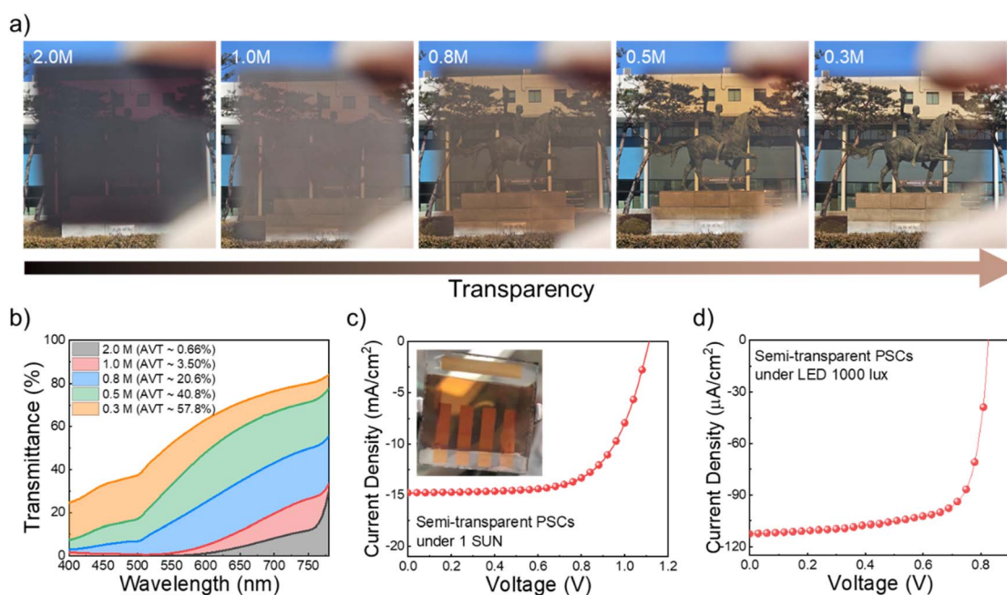
Fig. 6 (a) Photograph images of antisolvent-free perovskite films. (b) Transmittance spectra of the perovskite films with different molar concentrations. J - V curve of PSCs with semi-transparent perovskite films under (c) 1 sun and (d) LED 1000 lux illumination. The inset shows a photograph of PSCs incorporating a transparent perovskite layer.
