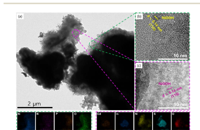
Fig. 6 (a) TEM image of the \text{NH}_4\text{NiPO}_4 \cdot \text{H}_2\text{O}/\text{CdIn}_2\text{S}_4/\text{Ni}_3\text{S}_2 heterostructure after the UOR process, highlighting the overall morphology and nanoscale features. (b and c) HRTEM images illustrating the formation of the \text{NiOOH} phase via surface reconstruction during UOR. The bottom panel displays TEM elemental mappings, confirming the uniform distribution of elements within the \text{NH}_4\text{NiPO}_4 \cdot \text{H}_2\text{O}/\text{CdIn}_2\text{S}_4/\text{Ni}_3\text{S}_2 heterostructure and validating the formation of \text{NiOOH} at the reconstructed regions.
