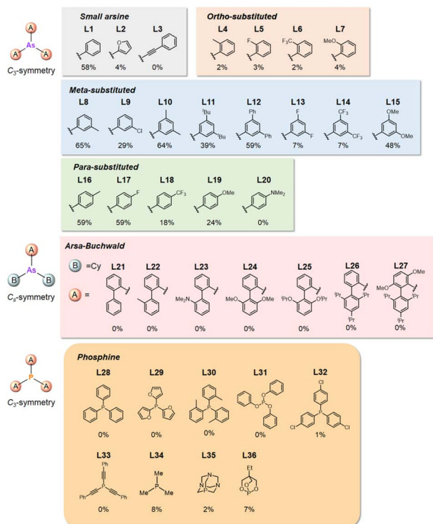
Fig. 2 o -, m -, and p -substituted C_{3-} and C_{2-} -type arsine and phosphine ligands. The NMR yield of the difunctionalized product 1 (Scheme 1) is shown below each structure.
