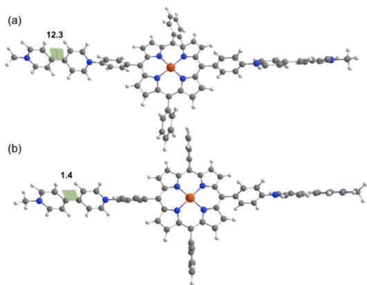
Fig. 2 Structural and electronic changes computed for (a) [(DV 2+ PP)Fe II ] + and (b) the corresponding two-electron reduced form best described as uncoupled two radical cations of the viologen and the Fe II porphyrin, [(DV + PP)Fe II ] 2+ . Numbers denote dihedral angles between pyridyl rings of viologen.
