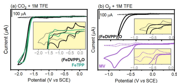
Fig. 3 Cyclic voltammograms of 0.25 mM (FeDVPP) 2 O (black) in DMF with 0.1 M [Bu 4 N]PF 6 and 1 M trifluoroethanol (TFE) under (a) CO 2 and (b) O 2 , in comparison to 0.5 mM FeTPP (green) and 0.5 mM MV (purple). Dotted curves show CV curves recorded in Ar-saturated DMF. Insets show zoomed data.
