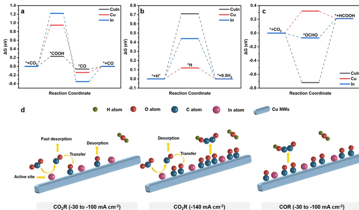
Fig. 5 Free-energy diagrams for (a) \text{CO}_2 to \text{CO} , (b) \text{H}_2 evolution, and (c) \text{CO}_2 to \text{HCOOH} on \text{CuIn} , \text{Cu} , and \text{In} surfaces. (d) Proposed mechanism for the formation of \text{CO} and \text{C}_{2+} products on the \text{CuIn} -30 catalyst under different conditions.
