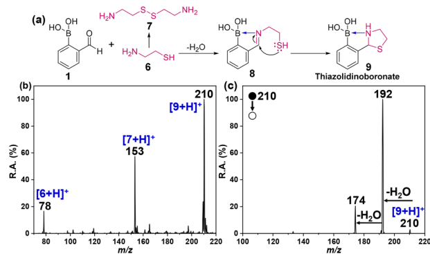
Fig. 4 (a) Formation of thiazolidinoboronate (9) via iminoboronate (8) in electrospayed microdroplets. (b) Positive mode nESI mass spectrum showing the product of the reaction between cysteamine and 2-FPBA in ACN microdroplets. Structures are shown for the labeled peaks. (c) MS/MS spectrum of the mass-selected thiazolidinoboronate product, [9+H] + , m/z 210, recorded using collision-induced dissociation (CID).
