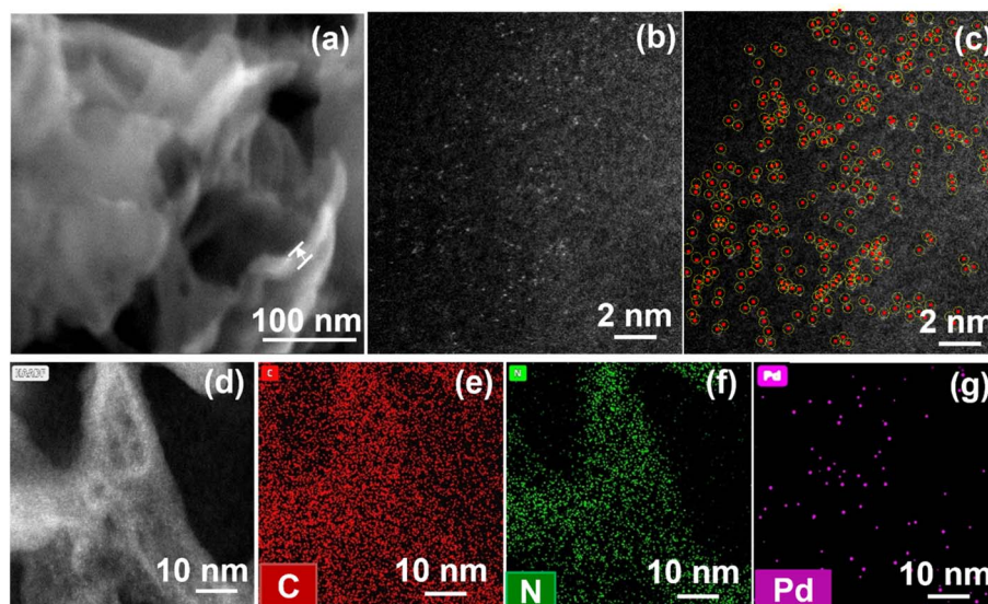
Fig. 1 (a) SEM image, (b) original HAADF-STEM image, (c) the HAADF-STEM image with individual Pd SAs highlighted by red dots and yellow circles, (d) HAADF-STEM image and the corresponding EDX mapping (e) C, (f) N, and (g) Pd of Pd SAs/C 3 N 4 .
