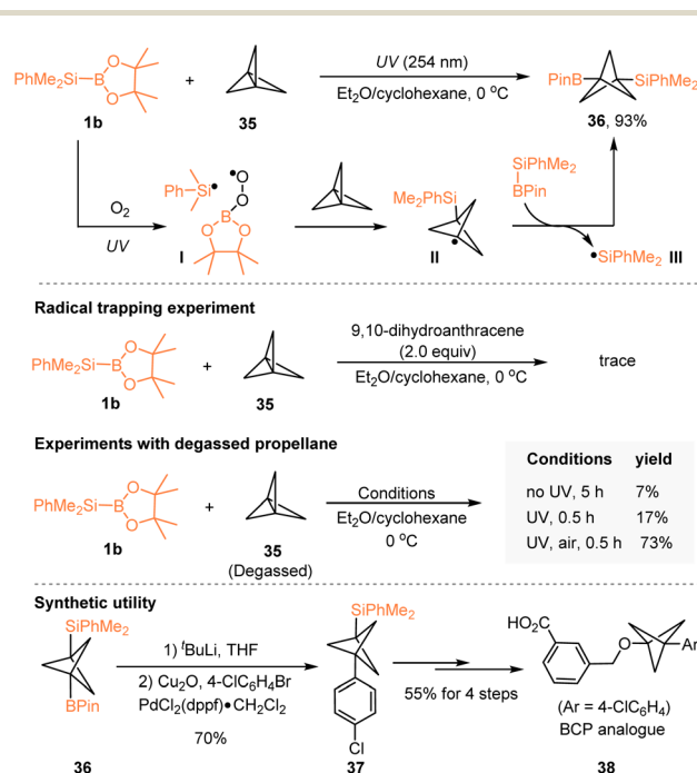
Scheme 11 Silaboration of [1.1.1]propellane with \text{PhMe}_2\text{Si-Bpin} .
