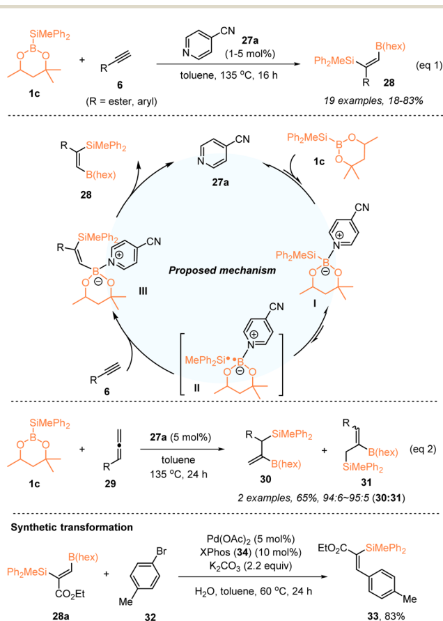
Scheme 10 Regioselective syn -1,2-silaboration of alkynes catalyzed by 4-cyanopyridine.
