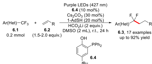
Scheme 6 Photoredox-organocatalyzed difluoro(hetero)arylation and difluoroalkylation of non-activated olefins.
