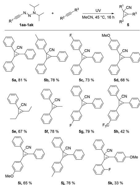
Scheme 10 Synthesis of cyclopropanes 5 with different alkynes and triazenes. 200 \mu\text{mol} triazene and 5.00 eq. alkyne in degassed MeCN (0.8 mL). Yields obtained after purification.
