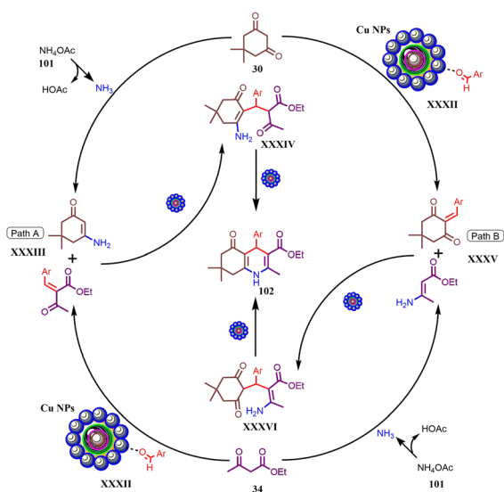
Fig. 11 Plausible mechanism for synthesis of hexahydroquinoline derivatives using an Fe 3 O 4 @SiO 2 @Si-(CH 2 ) 2 @HMAT@Cu nanocomposite (Salem et al. ).
