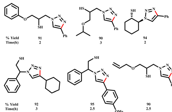
Scheme 5 \text{MgFe}_2\text{O}_4/\text{Cu} catalysed synthesis of \beta -thiol-1,4-disubstituted-1,2,3-triazoles from thiranes (Eisavi et al. ).
