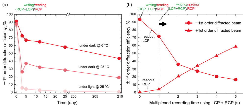
Fig. 5 (a) Retention ratio of -1\text{st} order diffraction efficiency for thin circular polarization hologram at various storage conditions. (b) Variation of \pm 1\text{st} order diffraction efficiency with different recording times of the second hologram for polarization hologram multiplexing.
