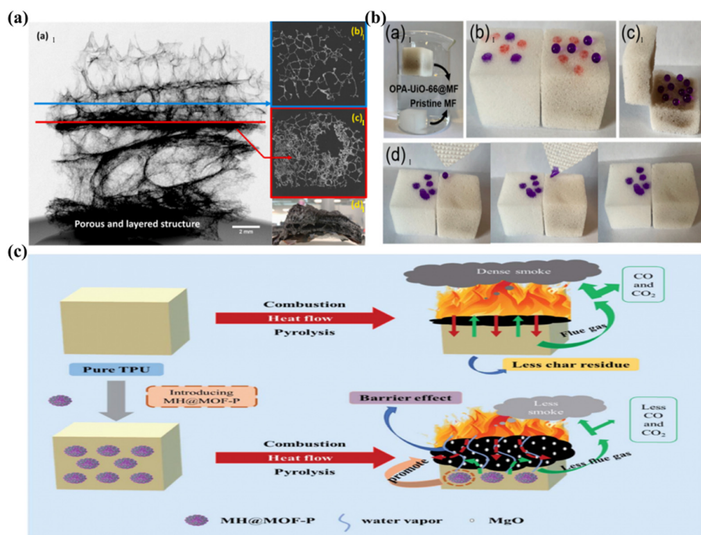
Fig. 6 (a): Results of X-ray tomography of EP composites with 7% \beta CD@P-MOF (a 1 ), with the selected layer at loose (b 1 ) and accumulated (c 1 ), digital photo of the cross-section view of the cut char residue (d 1 ). Reproduced from ref. 75 with permission from [Elsevier], copyright [2021]; (b): (a 1 ) MF sponge and OPA-UiO-66@MF in water; (b 1 ) n -hexane (red dyed) and water (purple dyed) droplets on MF sponge (left) and OPA-UiO-66@MF (right); (c 1 ) the wetting behaviors of the water droplets on the cross section of OPA-UiO-66@MF; (d 1 ) the wetting behaviors of the droplets on MF sponge and OPA-UiO-66@MF. Reproduced from ref. 82 with permission from [Elsevier], copyright [2022]; (c): Schematic illustration of flame retardant mechanism of TPU composites with MOF@MH-P. Reproduced from ref. 83 with permission from [The Royal Society of Chemistry], copyright [2021].
