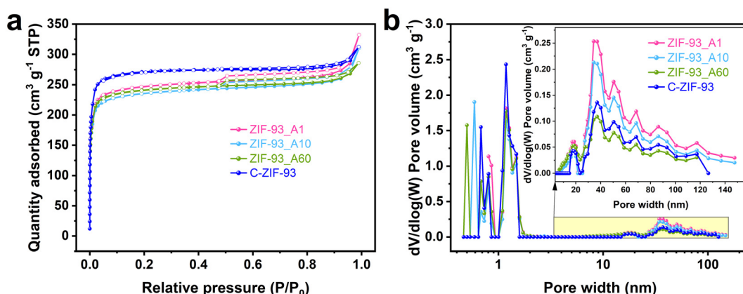
Fig. 4 (a) N 2 adsorption–desorption isotherms and (b) pore size distributions of ZIF-93_A1 and C-ZIF-93 samples.
