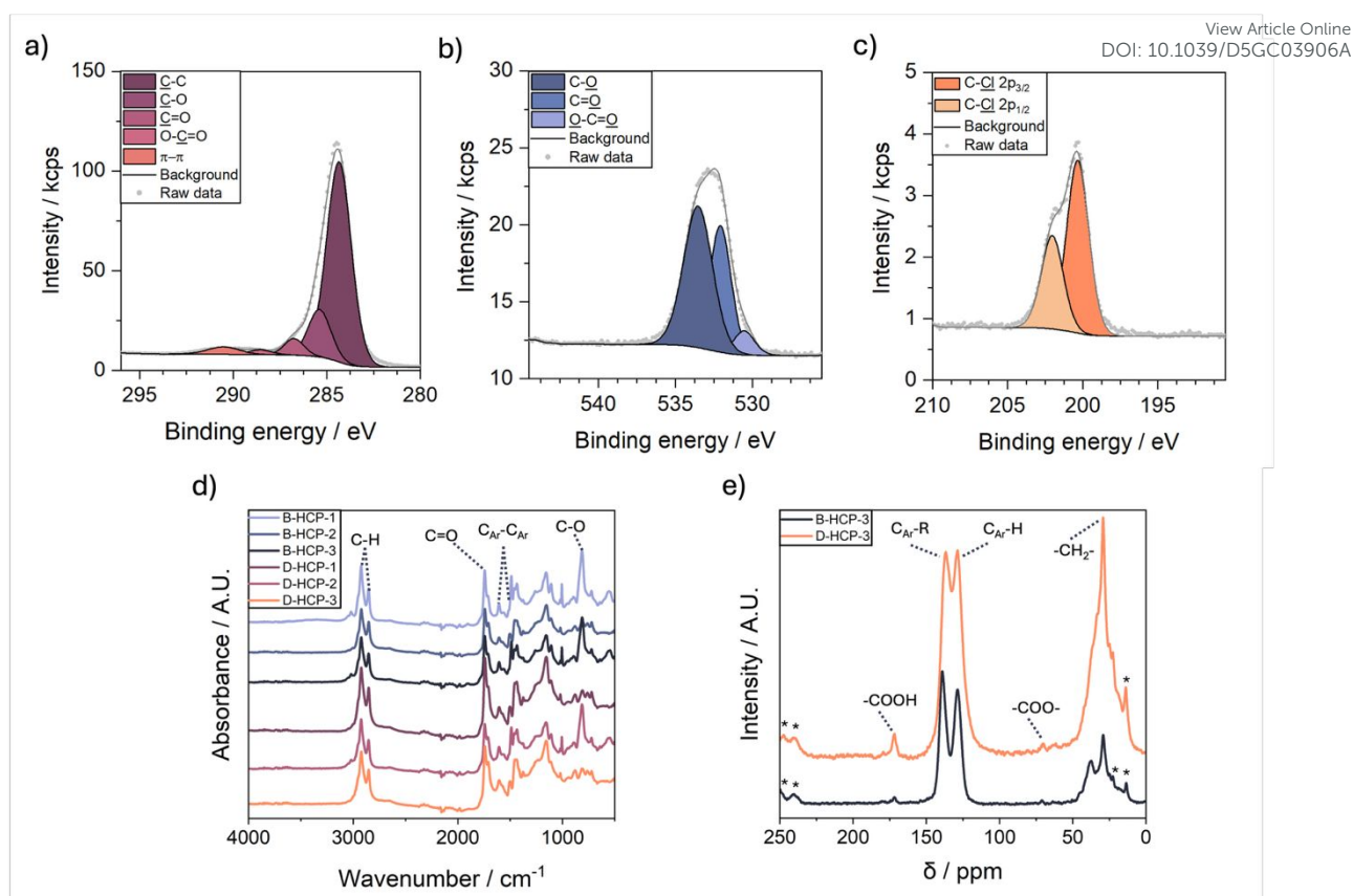
Figure 2. a) B-HCP-3 high-resolution C 1s XPS spectrum, b) B-HCP-3 high-resolution O 1s XPS spectrum, c) B-HCP-3 high-resolution Cl 2p spectrum, d) FTIR spectra of all B-HCPs and D-HCPs, e) ^{13}\text{C} cross-polarisation/magic angle spinning solid-state NMR of B-HCP-3 and D-HCP-3. * Represents spinning side bands.
