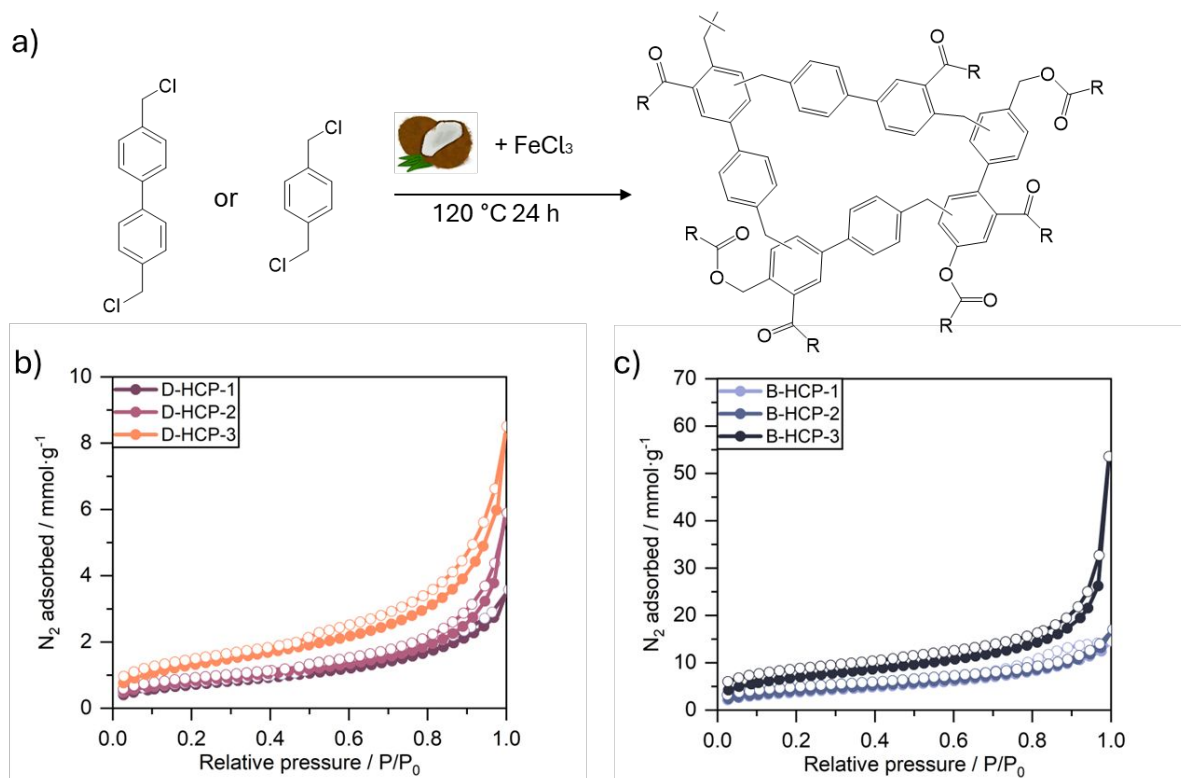
Figure 1. a) Representative reaction scheme for the synthesis of HCPs using coconut oil solvent. b) \text{N}_2 adsorption-desorption isotherms of D-HCPs, and c) B-HCPs.
