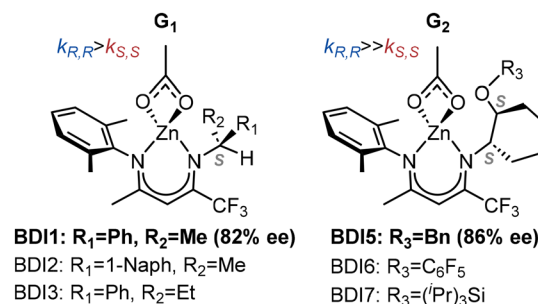
Scheme 2 Structures of G 1 and G 2 generations of zinc β-diiminate catalysts for enantioselective ROCOP of CHO and CO 2 . 12d
