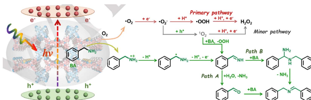
Fig. 14 Reaction mechanism of the photocatalytic H 2 O 2 production and BBAD co-production system. Reproduced with permission. 145 Copyright 2024, Wiley-VCH.
