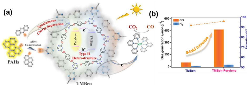
Fig. 13 (a) Schematic illustration of the PAH-functionalized TMBen for photocatalytic CO 2 reduction. (b) A comparison of the amount of product obtained with TMBen and TMBen–perylene after 5 hours of reaction. Reproduced with permission. 130 Copyright 2022, Wiley-VCH.
