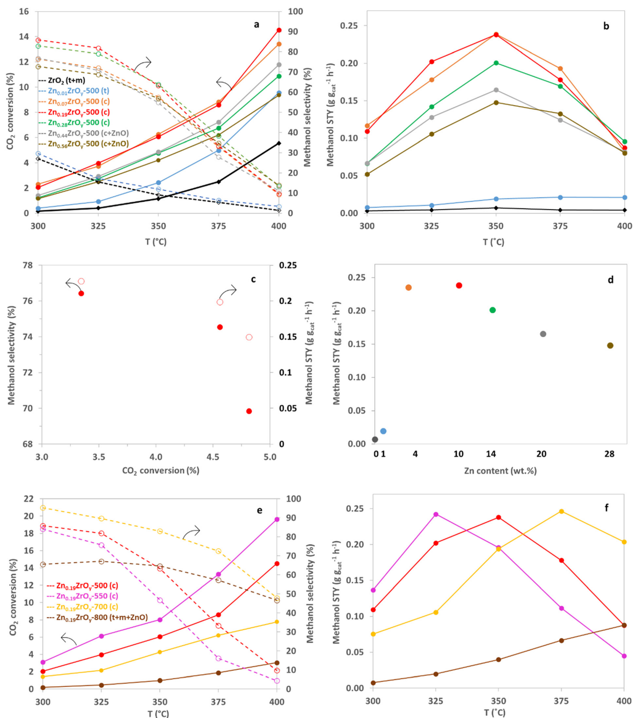
Fig. 8 Effect of temperature on (a) CO 2 conversion and methanol selectivity and (b) methanol STY of Zn x ZrO y -500 catalysts, at 45 bar, H 2 :CO 2 :Ar = 3:1:1, and GHSV = 21000 Nml g cat -1 h -1 . (c) Methanol selectivity versus CO 2 conversion on Zn 0.19 ZrO y -500 at 325 °C, 45 bar, H 2 :CO 2 :Ar = 3:1:1, and GHSV = 31500, 21000, and 15750 Nml g cat -1 h -1 . (d) Effect of Zn loading on methanol STY at 350 °C, 45 bar, H 2 :CO 2 :Ar = 3:1:1, and GHSV = 21000 Nml g cat -1 h -1 . (e) Effect of temperature on CO 2 conversion and methanol selectivity and (f) methanol STY of Zn 0.19 ZrO y -T catalysts, at 45 bar, H 2 :CO 2 :Ar = 3:1:1, and GHSV = 21000 Nml g cat -1 h -1 (full lines: CO 2 conversion-dotted lines: methanol selectivity).
