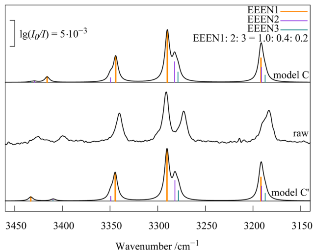
Fig. 10 Prediction of the spectrum of EEEN monohydrate based on (unscaled) harmonic calculations and the average calibration shifts and coupling constants obtained for the 8 other amine monohydrates discussed in this work, according to two coupling models. The predictions differ in the sequence of the two weak highest wavenumber transitions and the deviations of model C' are slightly more systematic than those of model C.
