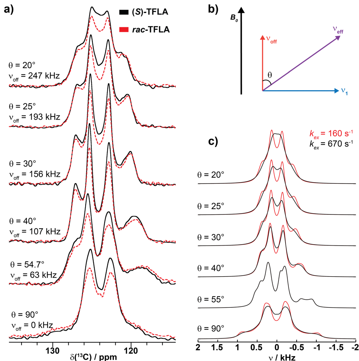
Fig. 5 (a) ^{19}\text{F} - ^{13}\text{C} CP spectra of the \text{CF}_3 spectral region for rac emic (dashed red curve) and ( S )-TFLA (straight black curve) recorded at 15.0 kHz MAS under off-resonance ^{19}\text{F} decoupling. The angle \theta of the effective ^{19}\text{F} field with respect to B_0 during CW decoupling varies as shown in the figure from 90^\circ to 20^\circ . (b) schematic representation for the calculations of the effective field during CW decoupling. (c) Numerical simulations of off-resonance ^{19}\text{F} decoupled spectra as a function of \theta and with k_{\text{ex}} = 160 \text{ s}^{-1} representing rac -TFLA and k_{\text{ex}} = 670 \text{ s}^{-1} representing ( S )-TFLA. The simulations are based on the following parameters: J(^{19}\text{F}-^{13}\text{C}) = -280 \text{ Hz} , J(^{19}\text{F}-^{19}\text{F}) = 100 \text{ Hz} , \delta(^{19}\text{F}-^{13}\text{C})/2\pi = 7870 \text{ Hz} , \delta(^{19}\text{F}-^{19}\text{F})/2\pi = 10700 \text{ Hz} , \delta_\sigma(^{19}\text{F})/2\pi = 26352 \text{ Hz} with all tensors oriented along the rotation axis of the \text{CF}_3 group. The MAS frequency was set to 15.0 kHz, B_1 to 90 kHz, and the offsets values as indicated in the figure.
